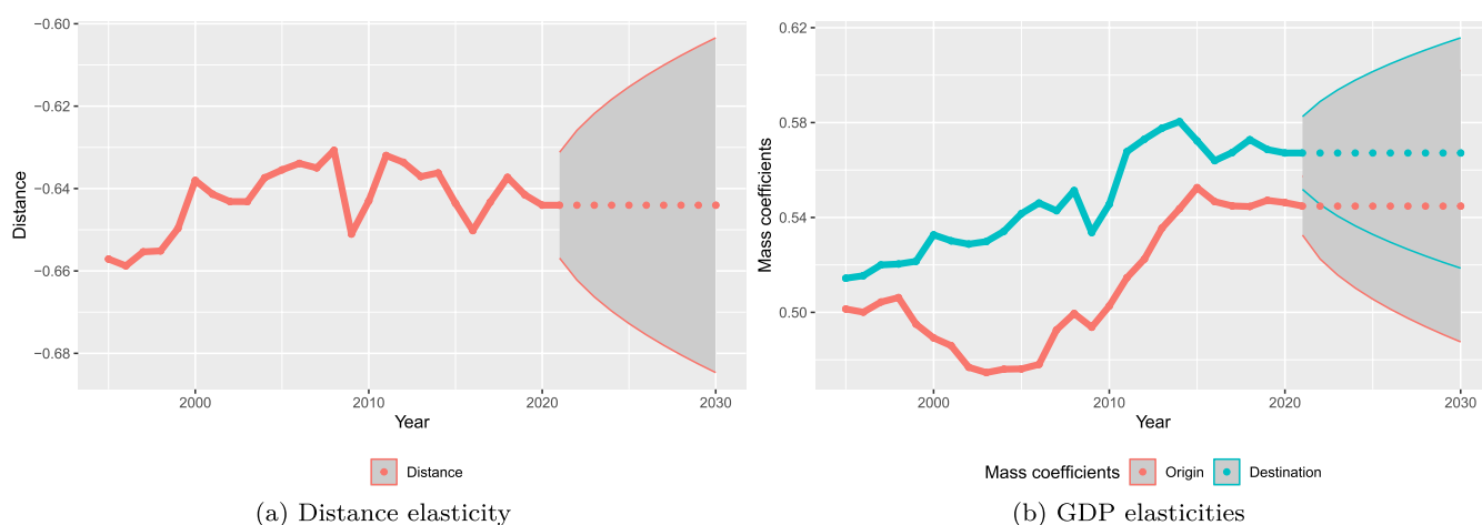
FIGURE 2 | Aggregate gravity coefficients from OECD-ICIO network (1995–2022) with ARIMA forecasts to 2030 (95% CI). [Colour figure can be viewed at wileyonlinelibrary.com ]
