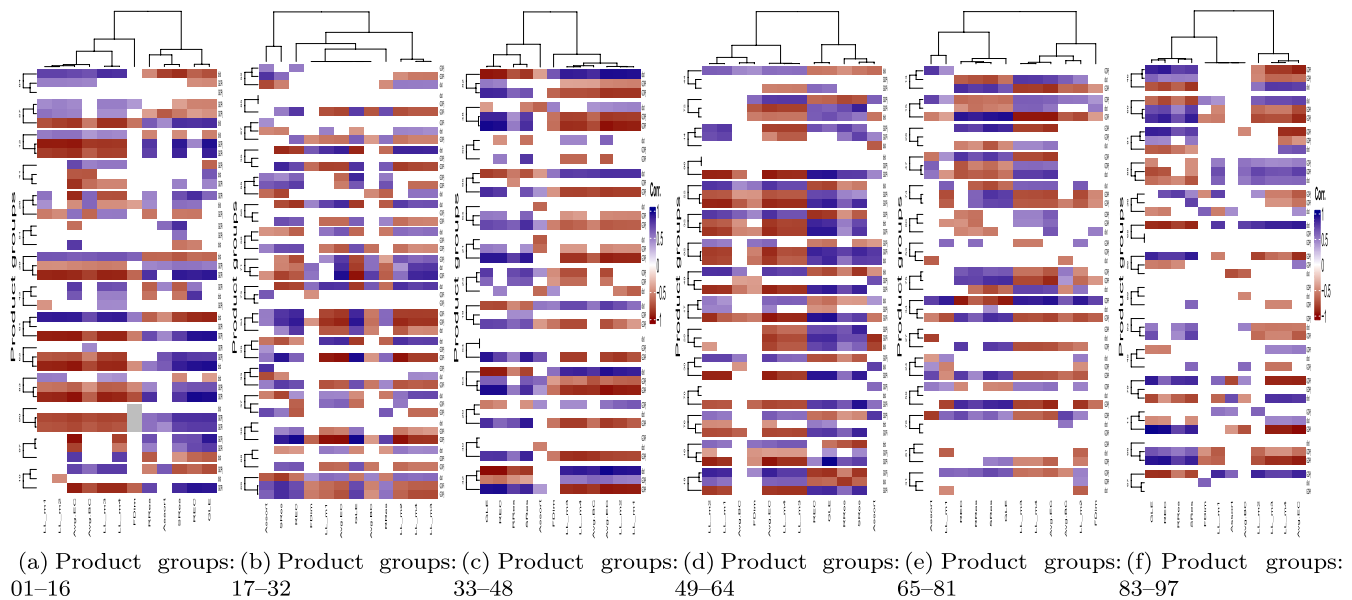
FIGURE A6 | Spearman's correlation between gravity coefficients and network-level (and aggregated node-level) indicators. [Colour figure can be viewed at wileyonlinelibrary.com ]
