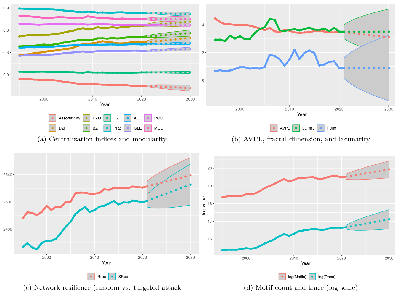
FIGURE 3 | Network-level properties (forecast with ARIMA, 95% confidence interval, based on OECD-ICIO database). [Colour figure can be viewed at wileyonlinelibrary.com ]
