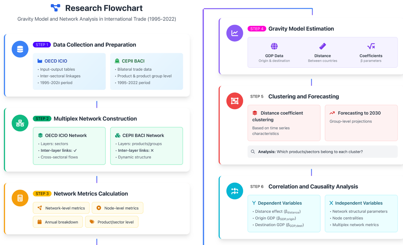
FIGURE 1 | Research flowchart. [Colour figure can be viewed at wileyonlinelibrary.com ]
