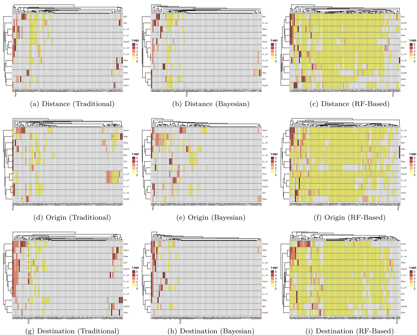
FIGURE 10 | Panel-based causality analysis for product groups (based on BACI-CEPII database). [Colour figure can be viewed at wileyonlinelibrary.com ]
