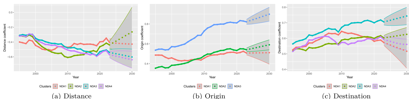
FIGURE A4 | Coefficients of gravity models for products in time (forecast with ARIMA, 95% confidence interval). [Colour figure can be viewed at wileyonlinelibrary.com ]
