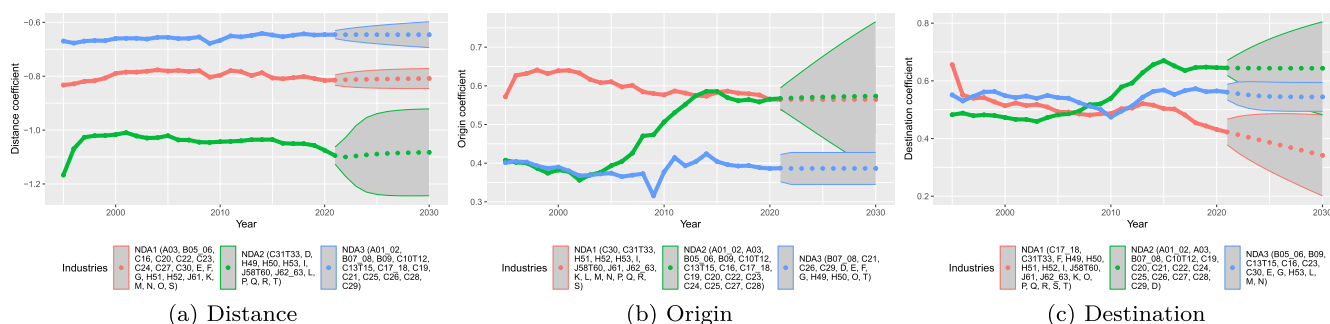
FIGURE A1 | Coefficients of gravity models in time (forecast with ARIMA, 95% confidence interval, based on OECD-ICIO database). [Colour figure can be viewed at wileyonlinelibrary.com ]
