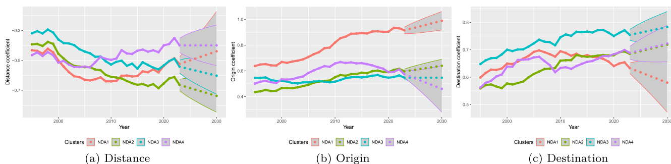
FIGURE A3 | Coefficients of gravity models for product subgroups in time (forecast with ARIMA, 95% confidence interval, based on BACI-CEPII database). [Colour figure can be viewed at wileyonlinelibrary.com ]
