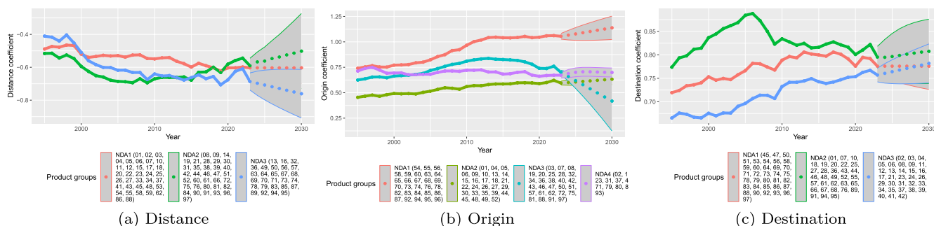
FIGURE A2 | Coefficients of gravity models for product groups in time (forecast with ARIMA, 95% confidence interval, based on BACI-CEPII database). [Colour figure can be viewed at wileyonlinelibrary.com ]
