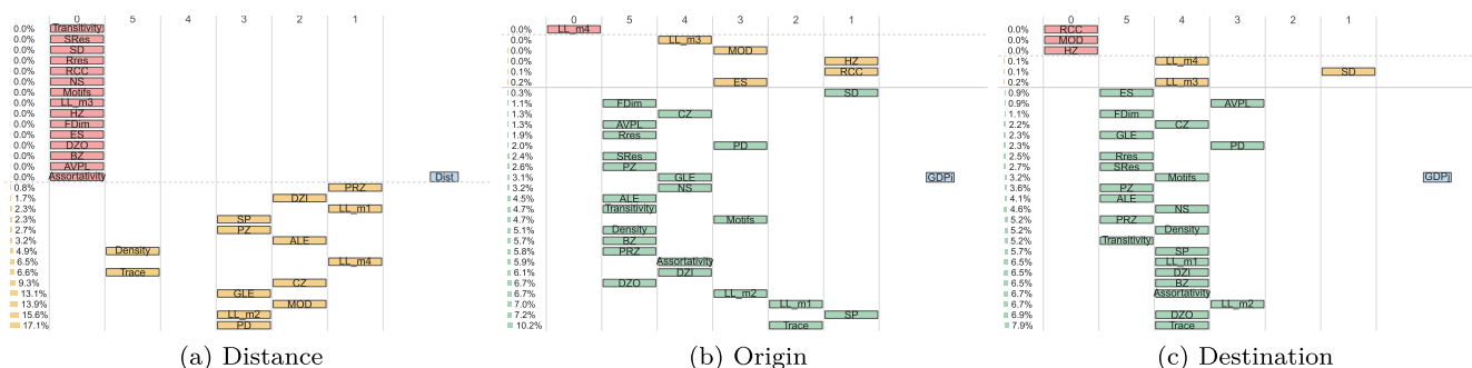
FIGURE 8 | Random Forest-Based Granger-Like Causality Analysis between gravity and multilayer network indicators (based on OECD-ICIO database). [Colour figure can be viewed at wileyonlinelibrary.com ]
