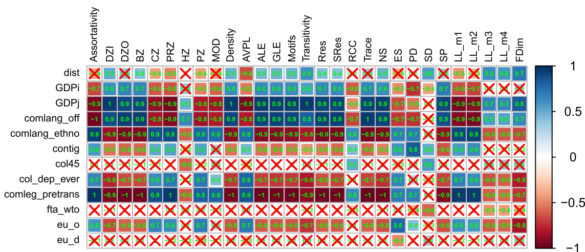
FIGURE 4 | Spearman's correlation between gravity coefficients and network-level (and aggregated node-level) indicators (based on OECD-ICIO database); cells marked with a red × are not statistically significant after Holm adjustment ( p_{adj} \geq 0.05 ). [Colour figure can be viewed at wileyonlinelibrary.com ]
