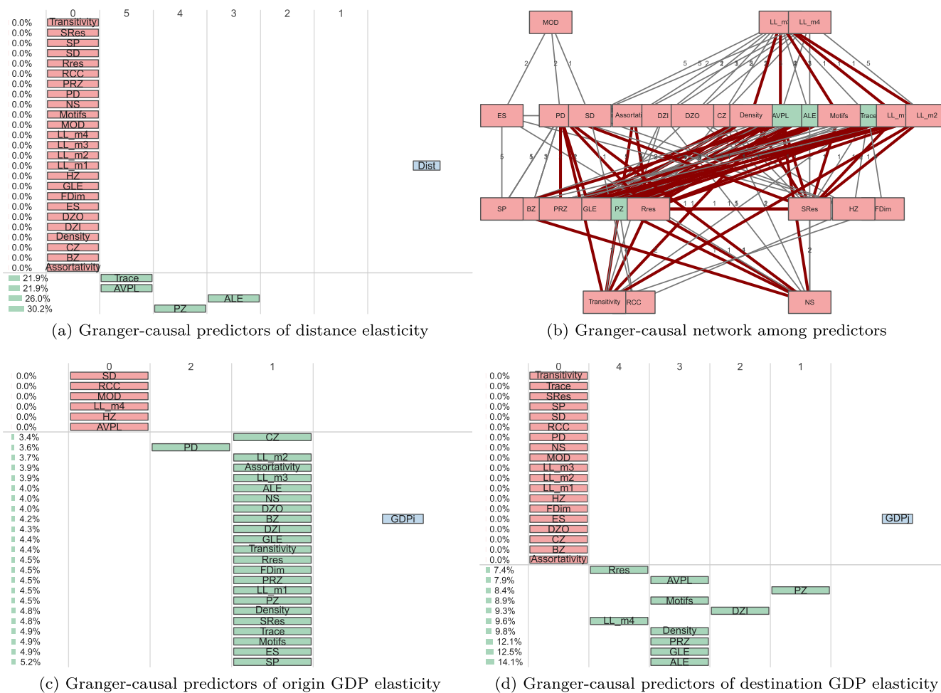
FIGURE 7 | Traditional Granger causality: From network indicators to gravity coefficients (OECD-ICIO aggregate). [Colour figure can be viewed at wileyonlinelibrary.com ]
