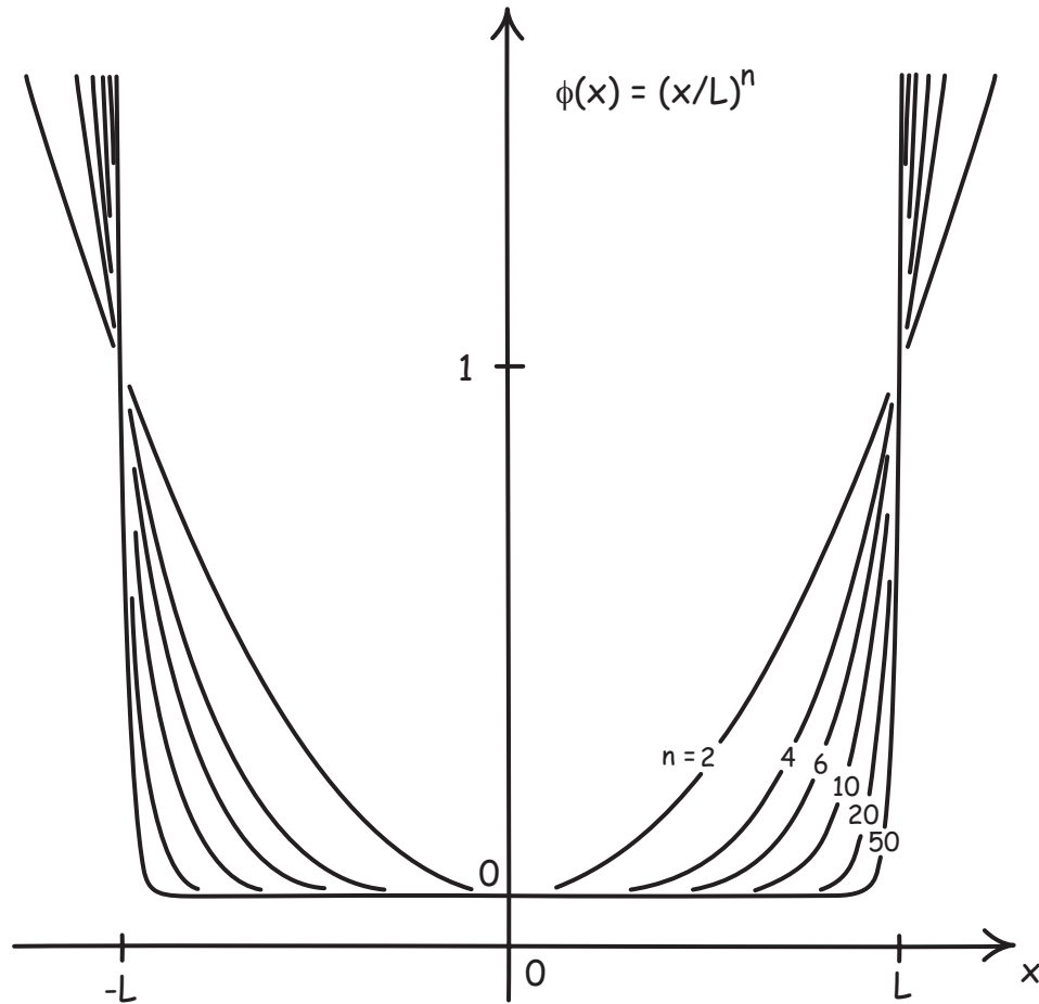
Figure 8. Analytic potential functions approach non-analytic limit.
