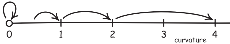
Figure 7. Space of sphere curvature.
