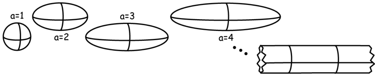
Figure 3. Sphere Elongated as Ellipsoid
